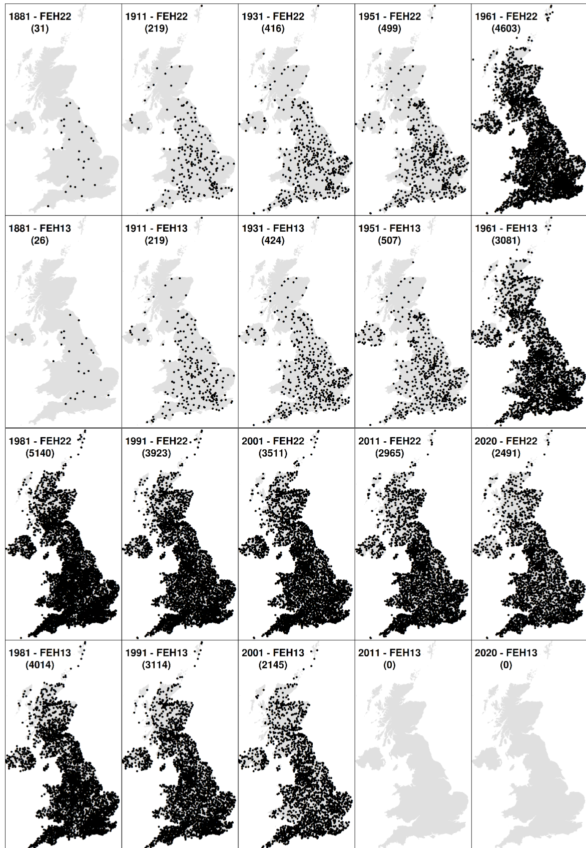
Figure 1 Spatial distribution of daily rainfall gauges used in FEH13 and FEH22 at individual years between 1881 and 2020.
