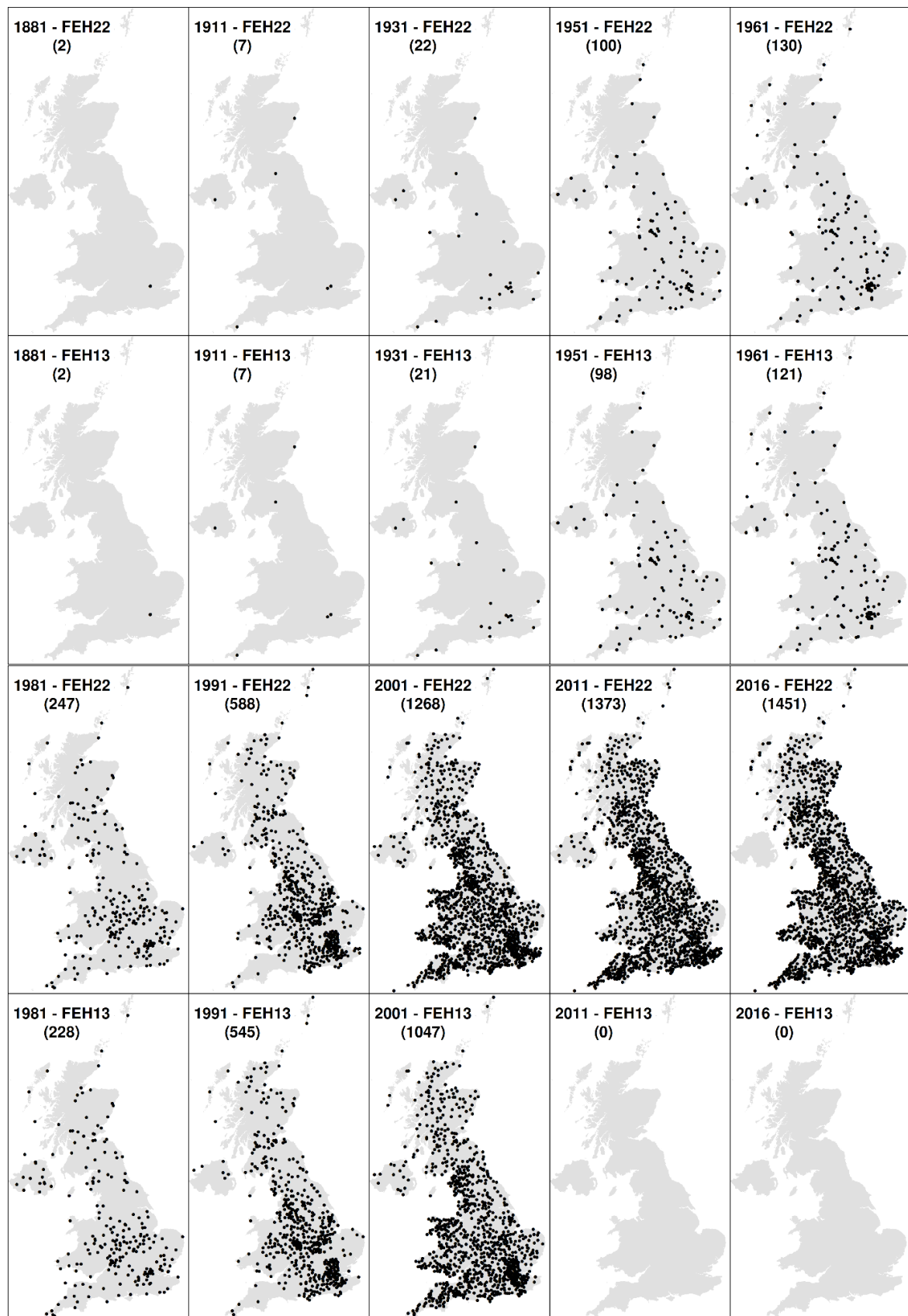
Figure 2 Spatial distribution of hourly rainfall gauges used in FEH13 and FEH22 at the individual years between 1881 and 2020.
