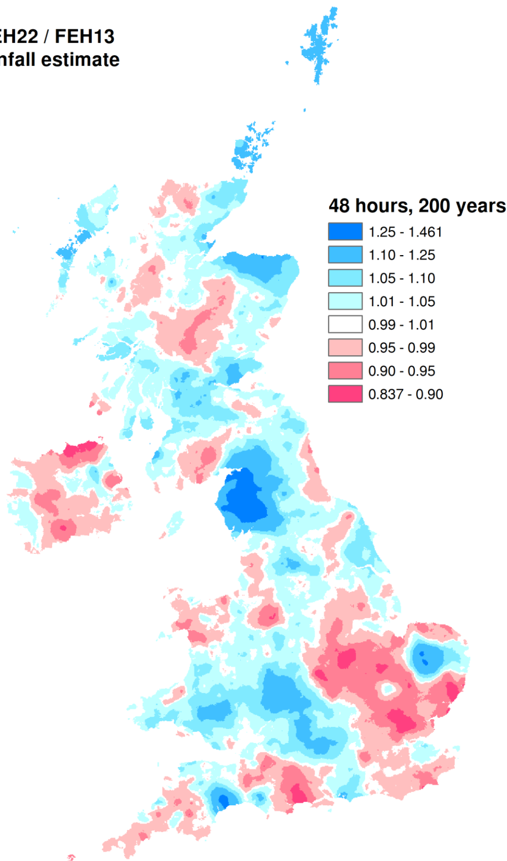
Figure 39 FEH22 rainfall depth as fraction of FEH13 rainfall depth: 48-hour, 200-year event.
