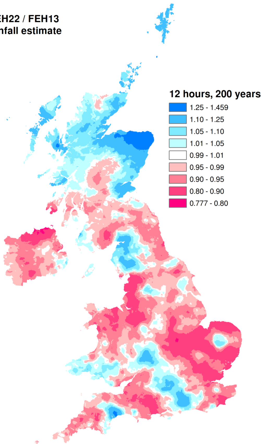
Figure 27 FEH22 rainfall depth as fraction of FEH13 rainfall depth: 12-hour, 200-year event.
