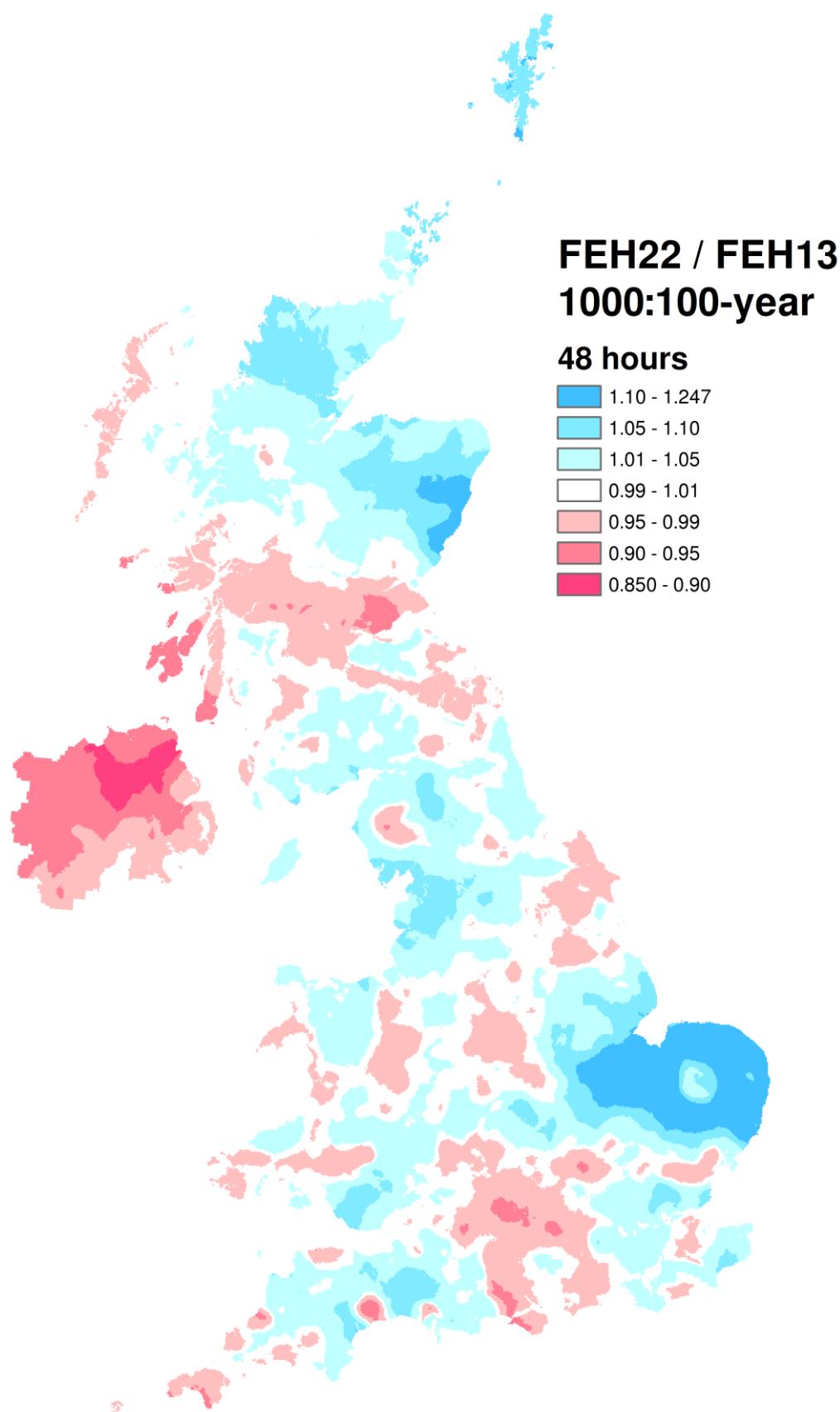
Figure 76 FEH22 1000:100-year rainfall depth as fraction of FEH13 1000:100-year rainfall depth: 48-hour.
